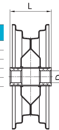
MOZZO CON BOCCOLE NYLON HUB WITH NYLON BUSHING
