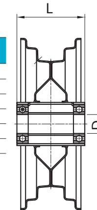
MOZZO CON CUSCINETTI A SFERA HUB WITH BALL BEARINGS
