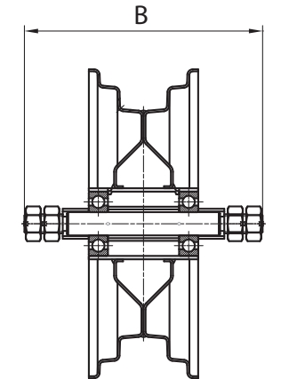
CUSCINETTI A SFERA + PERNO M14 BALL BEARINGS FORK AXLE M14
