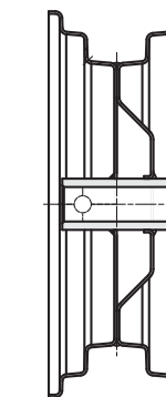
TUBO CILINDRICO FORO SPINA PIPE WITH TRACTION HOLE
